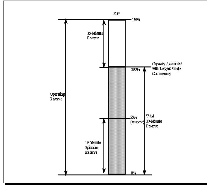
Figure 12: Operating Reserve Requirements
